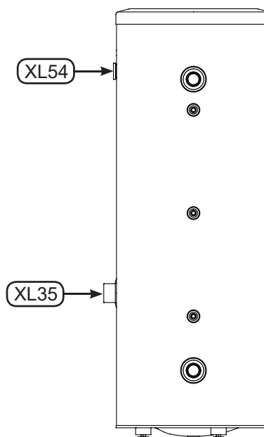
Fig. 6 Side view of the UKV 20-220 buffer tank.
