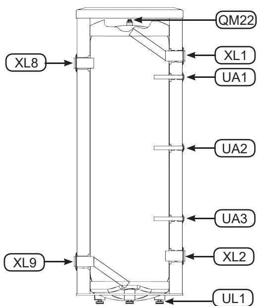
Fig. 4 Section of the UKV 20-220 buffer tank.
