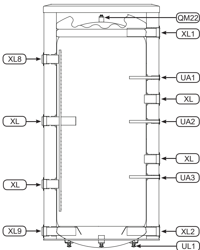
Fig. 8 Section of the UKV 20-750 and UKV 20-1000 buffer tank.
