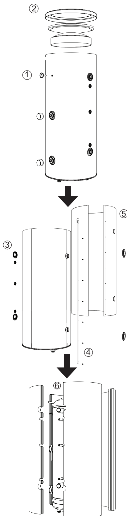
Fig. 11 Housing disassembly
