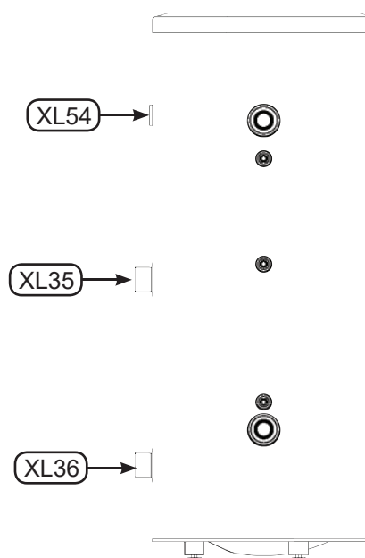
Fig. 7 Side view of the UKV 20-300 / 20-500 buffer tank.
