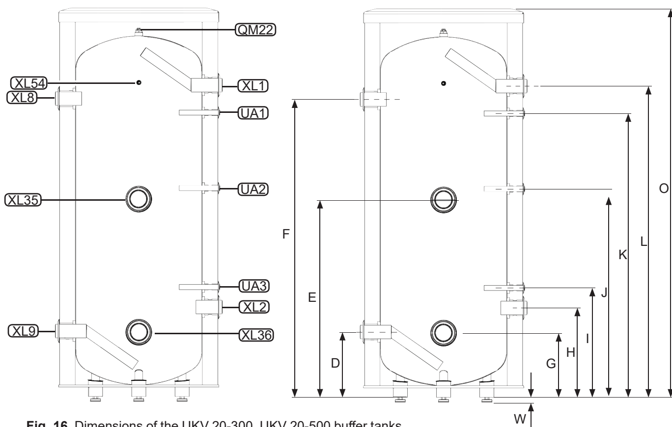
Fig. 16 Dimensions of the UKV 20-300, UKV 20-500 buffer tanks.
